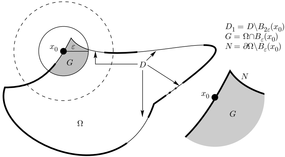
FIGURE 1. Geometric objects employed in the proof of strict monotonicity of \ell(A)
